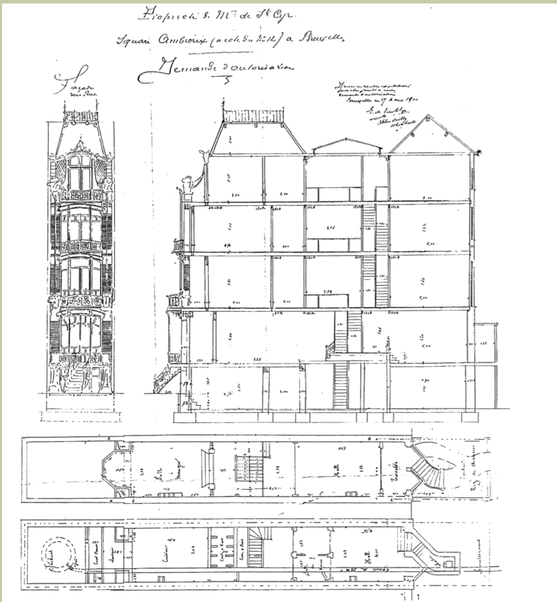
Elevation of the main facade - longitudinal section - Plan of the main floor
