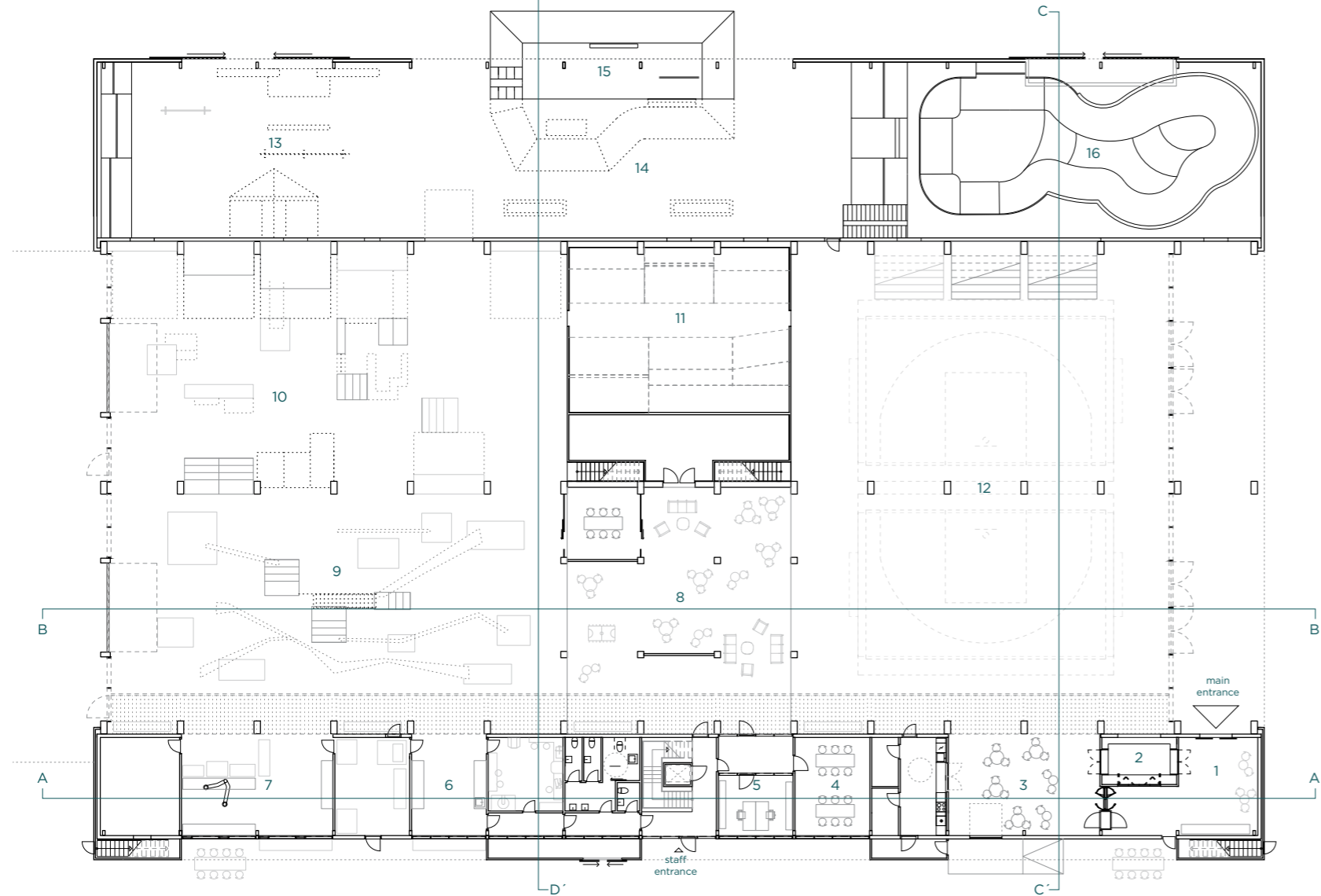
Ground floor
