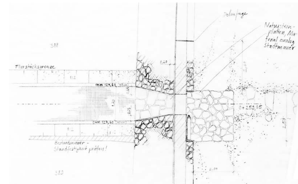
New City Wall with integrated flood barrier
