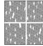
Concrete pavement with a very high proportion of 15/25mm aggregate (aggregate incorporated into the surface)
