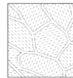
Bush-hammered natural limestone pavement. Thickness: 6-8cm Joint: 1-5cm. Irregular joint shape.
